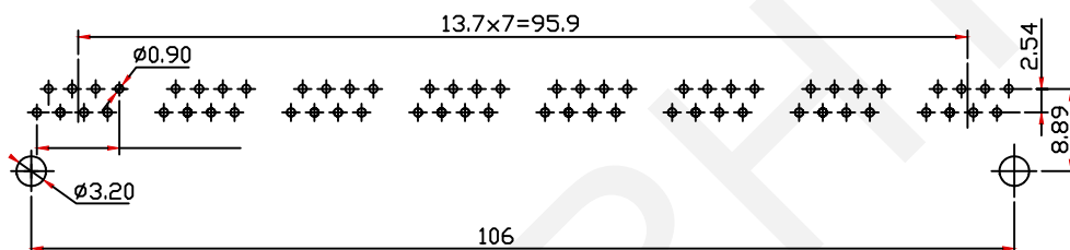
PCB Layout
